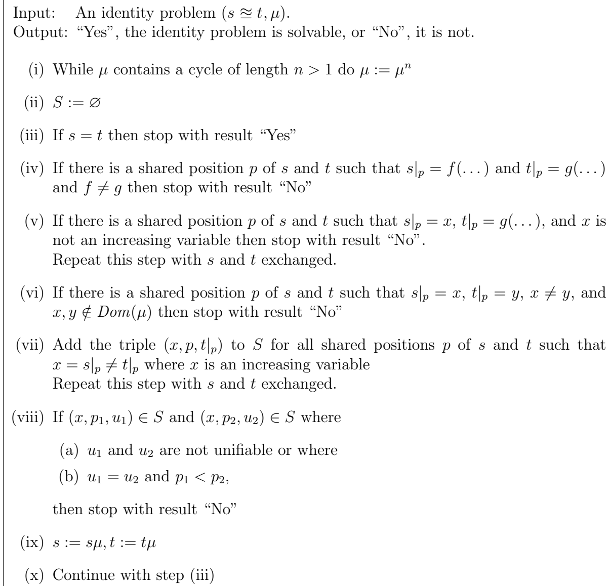
Figure 8.19.: An algorithm to decide solvability of identity problems
