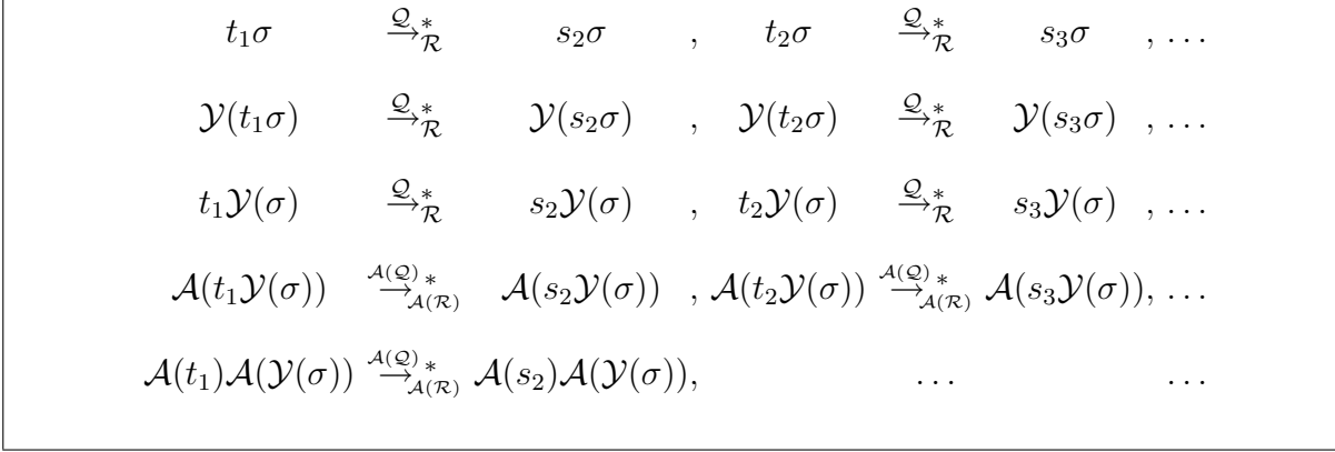
Figure 6.7.: Transformation of chains
