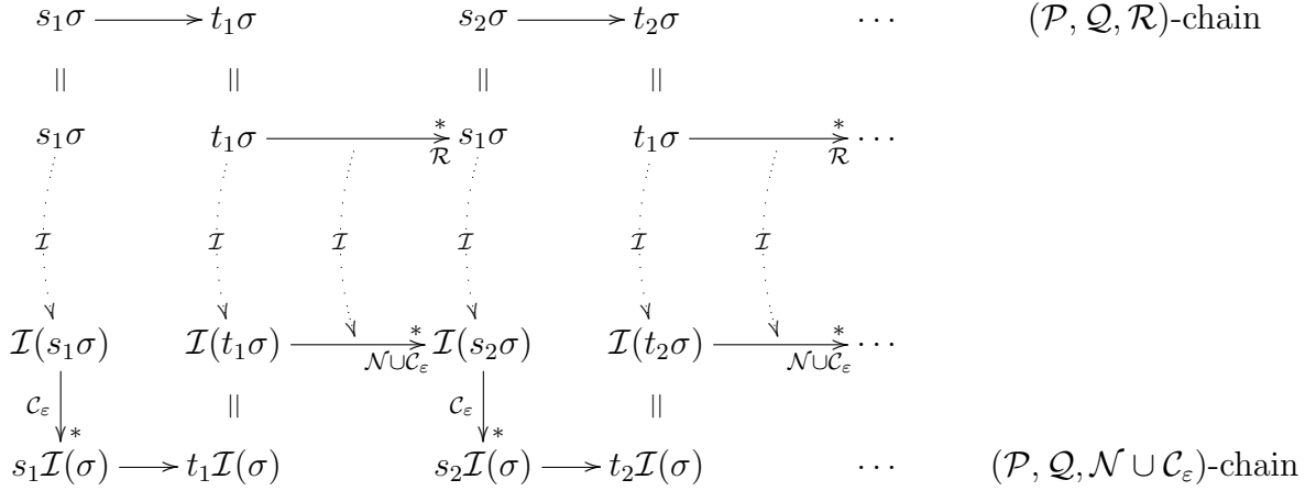
Figure 4.8.: Transformation of chains
