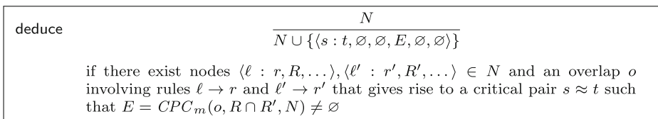
Fig. 7 The deduce inference rule using a critical pair criterion
