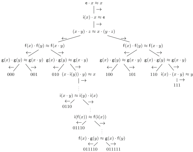
Fig. 5 Part of a CGE 2 process tree with all branching points leading to process 011110
